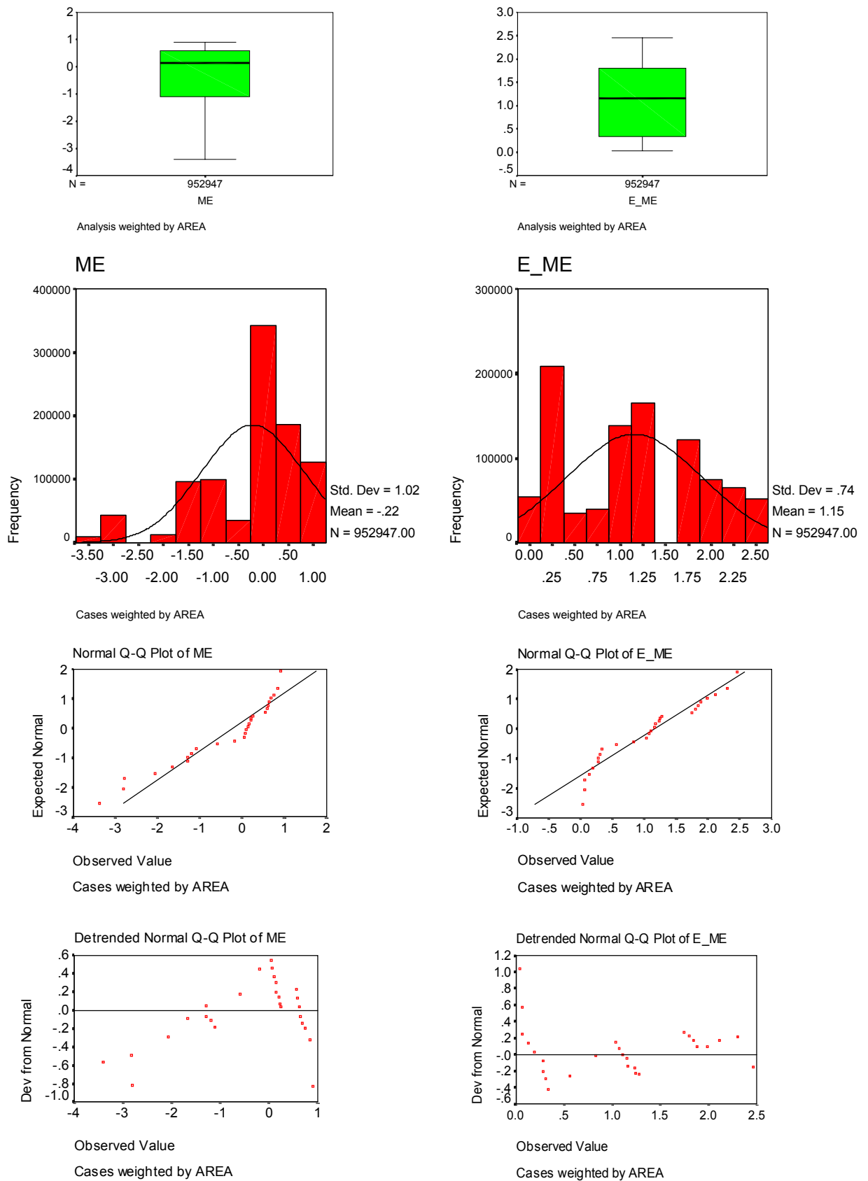
Figure 5-26: Explorative analysis of model efficiencies of all test catchments except for the Kymijoki and Júcar basins. Left: variable ME, right: variable e^{ME} . a) Boxplot, b) Histogram with normal curve, c) Normal Q-Q-Plot, d) Detrended normal Q-Q-Plot. The analysis is carried out for the model run resulting in a maximum \overline{ME}_{all} (see Table 5-2).
