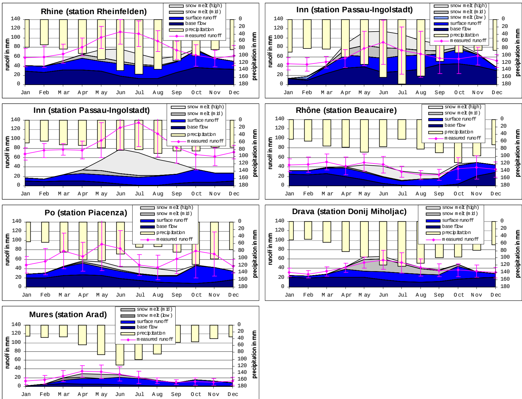
Figure 5-16: Observed and predicted runoff of the test catchments within runoff regime class 1 (monthly means 1961-90).
