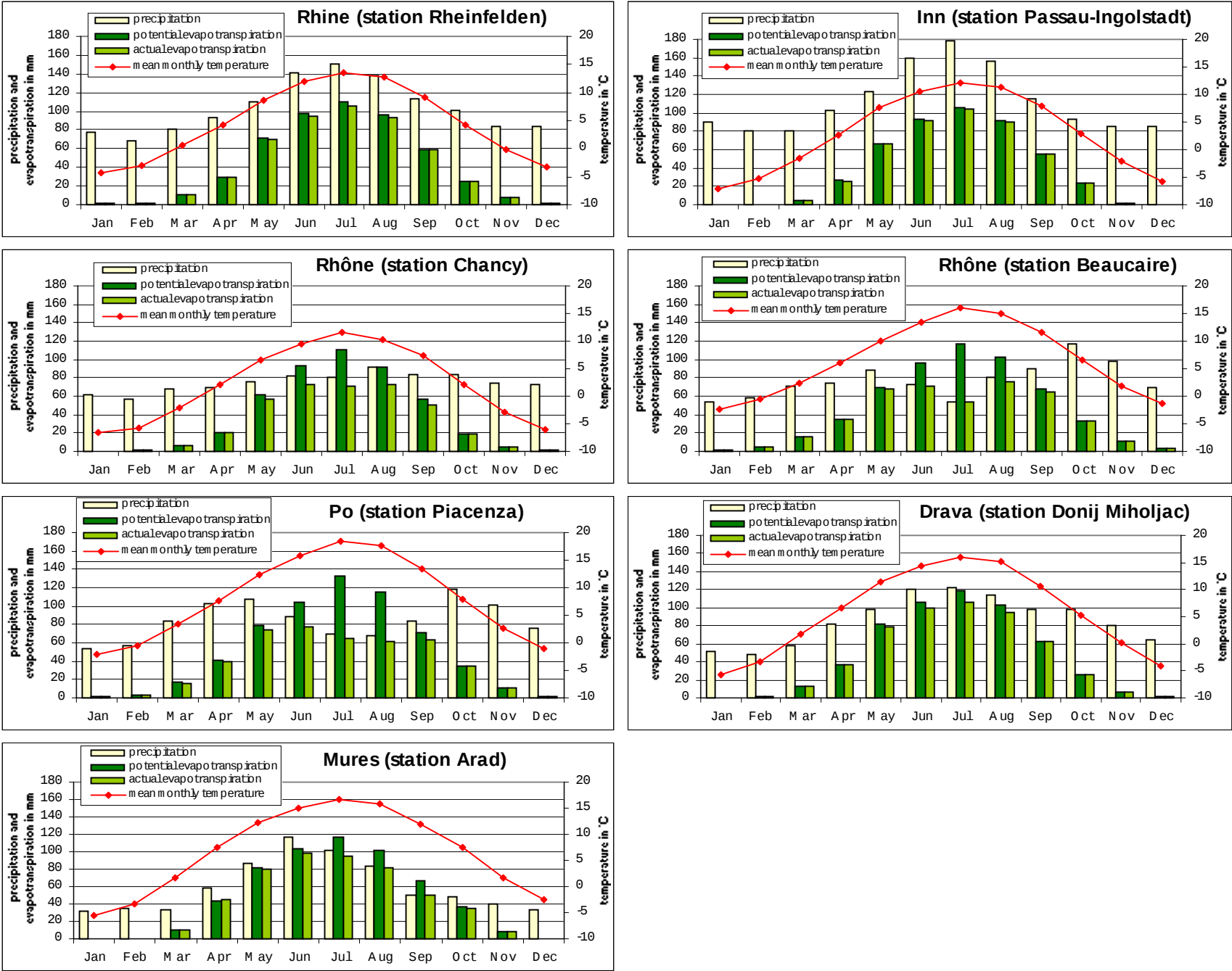
Figure 5-17: Temperature and precipitation as input data and potential and actual evapotranspiration as model results of the test catchments within runoff regime class 1 (monthly means 1961-90).
