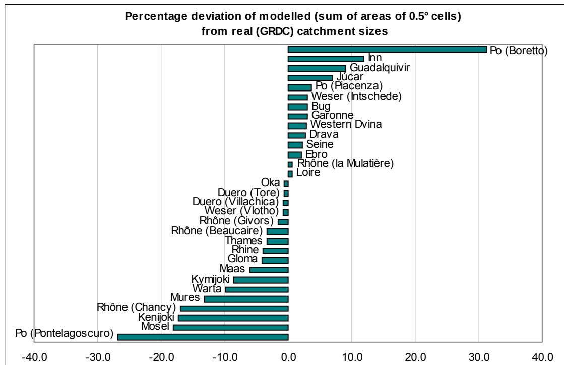
Figure 4-4: Percentage deviation of modelled (sum of areas of 0.5° cells) from real catchment sizes.
