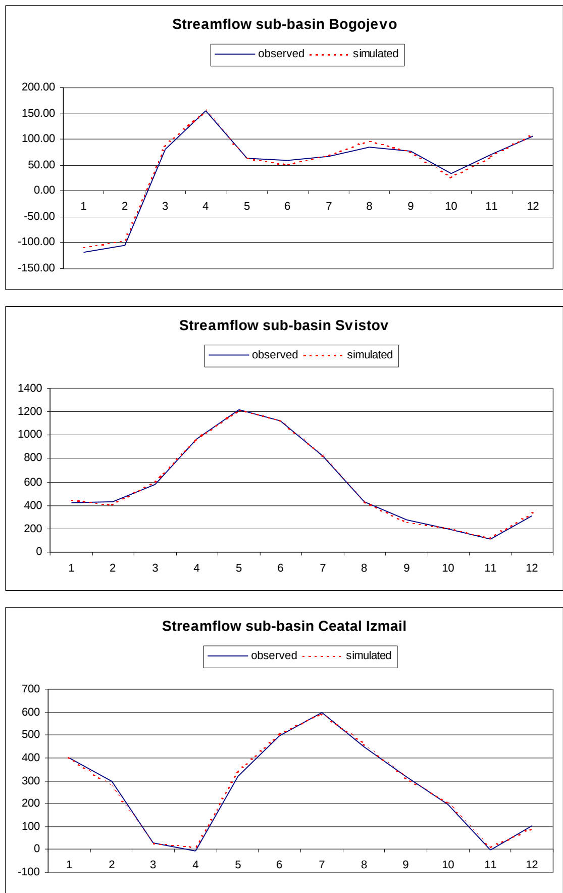
Figure 10 j-l: Comparison of simulated and observed monthly streamflow
