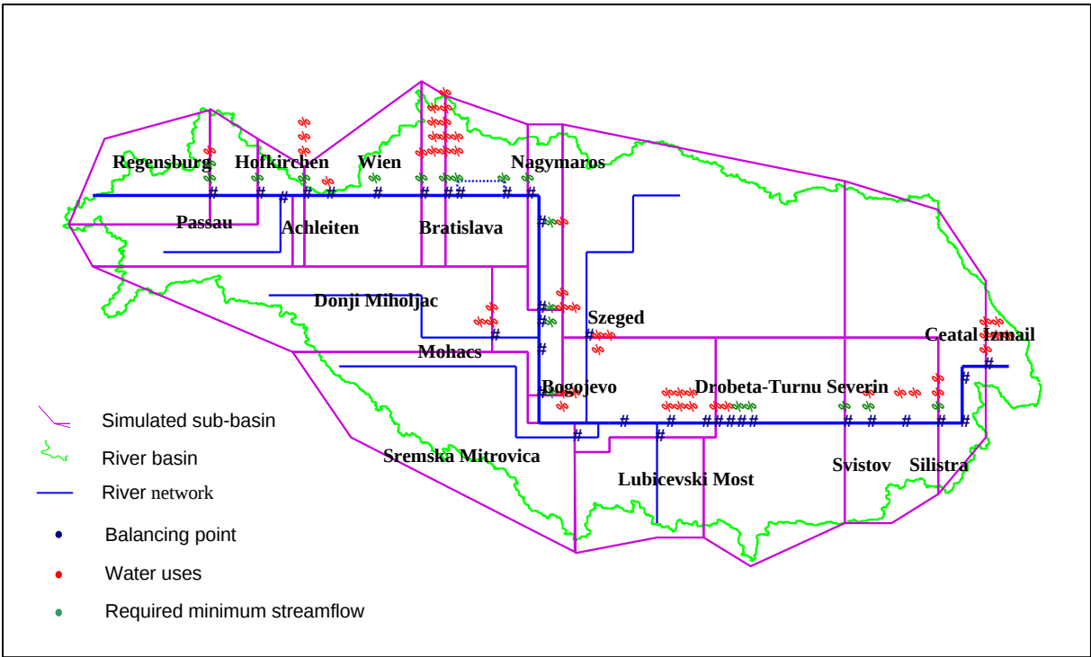
Figure 20: Water uses
