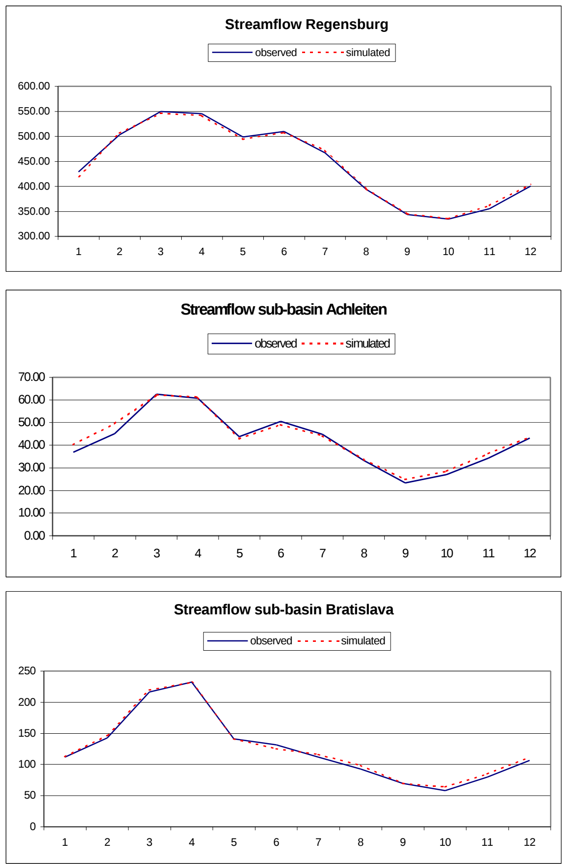
Figure 10 a-c: Comparison of simulated and observed monthly streamflow
