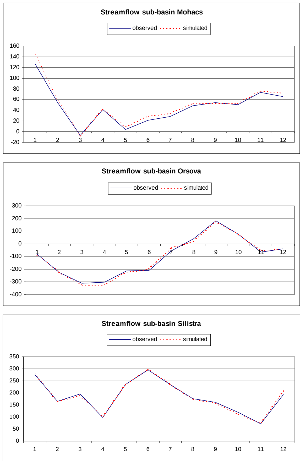
Figure 10 g-i: Comparison of simulated and observed monthly streamflow
