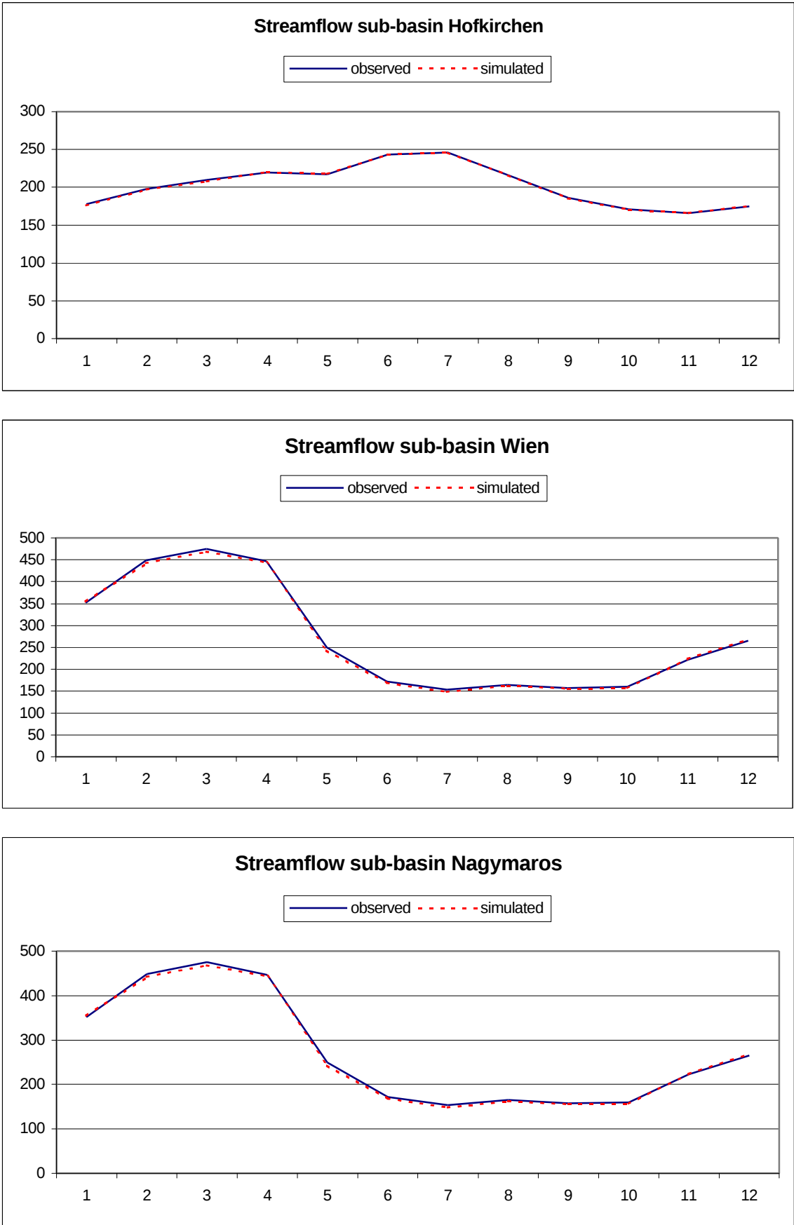
Figure 10 d-f: Comparison of simulated and observed monthly streamflow
