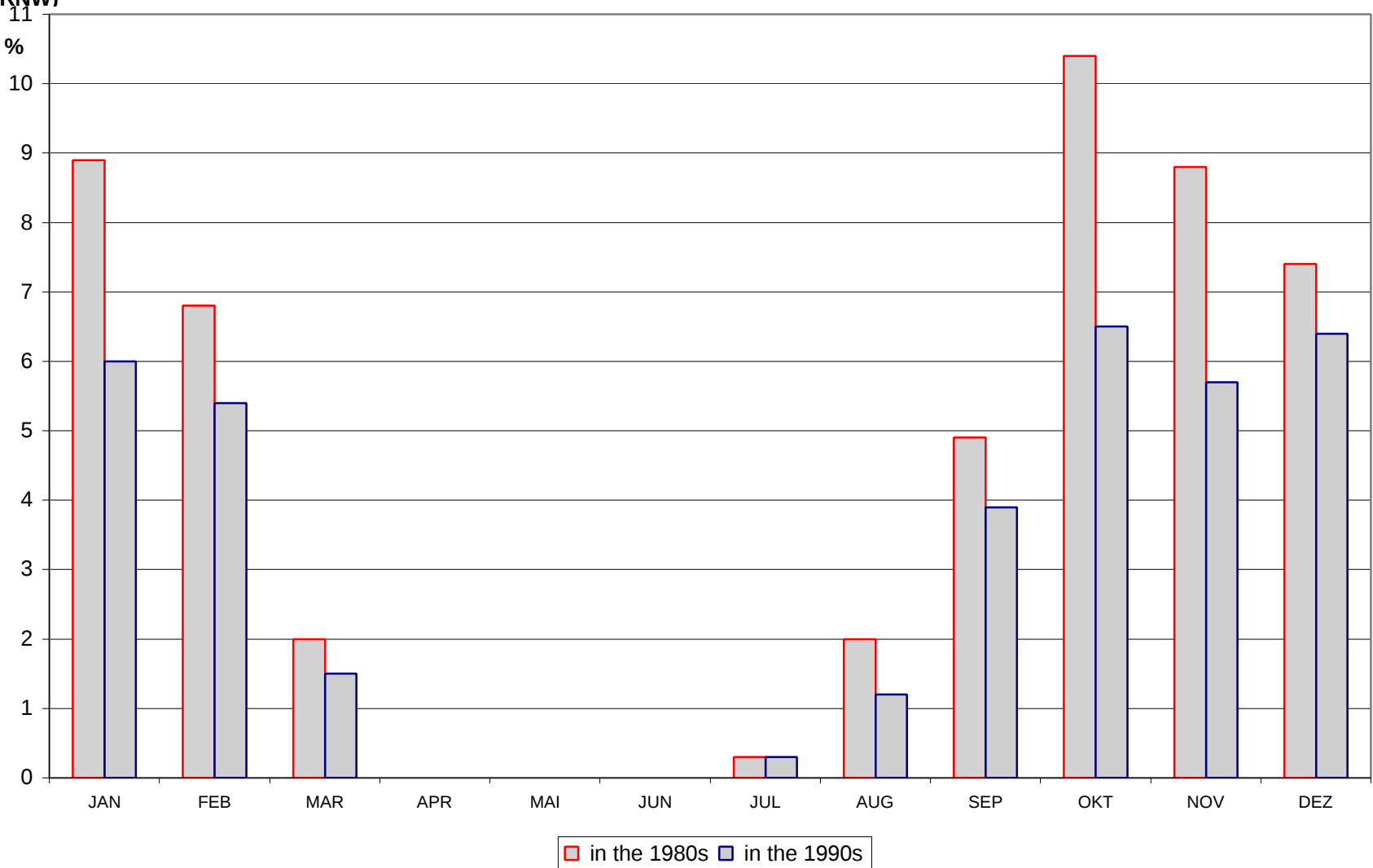
Figure 28b: Frequency of the monthly non-exceedance of minimum navigational streamflow QRNW at Mohacs in comparison (MQmon < ORNW)
