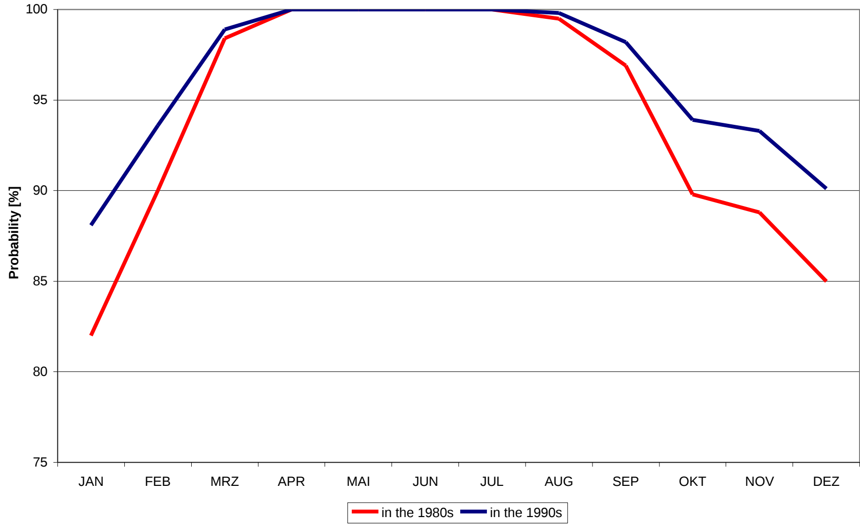
Figure 27a: Exceedance of minimum navigational streamflow Q_{RNW} at Bratislava in comparison
