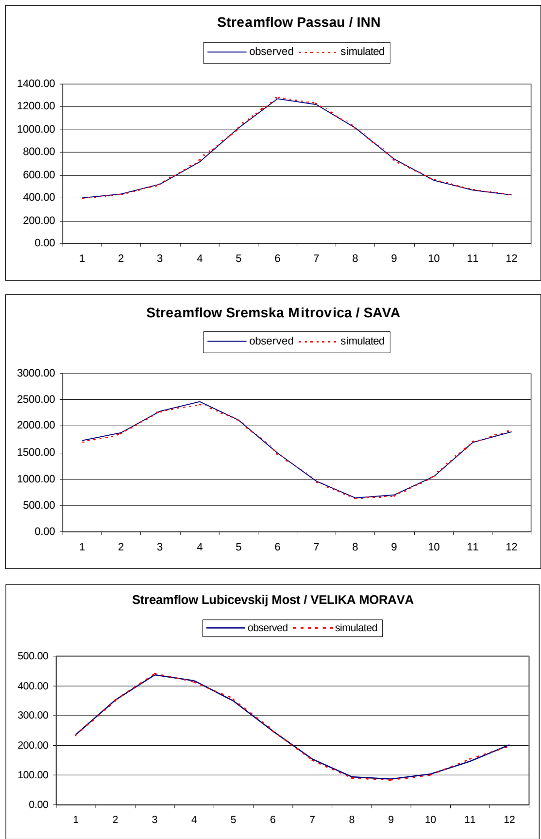
Figure 10 m-o: Comparison of simulated and observed monthly streamflow
