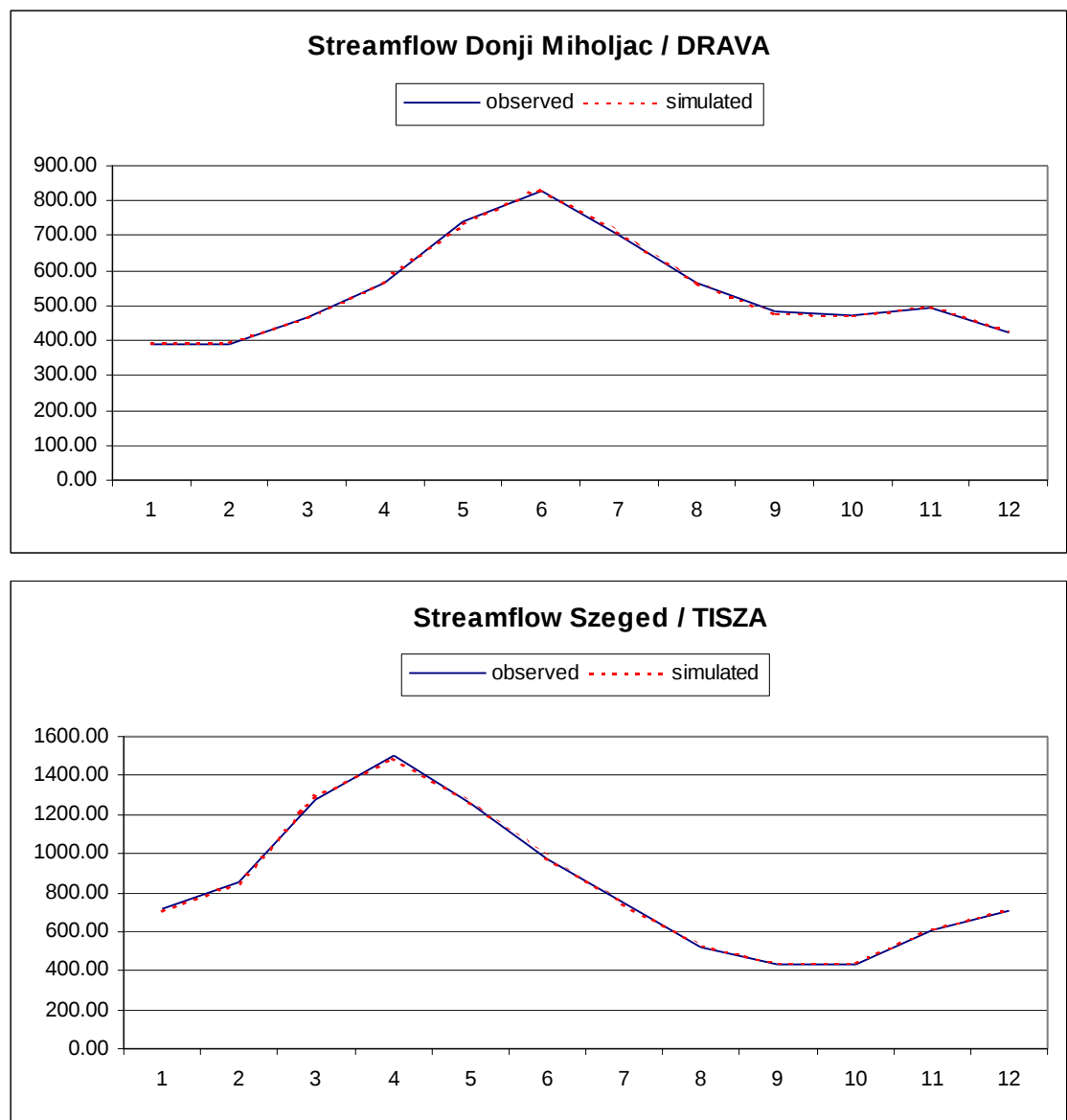
Figure 10 p-q: Comparison of simulated and observed monthly streamflow
