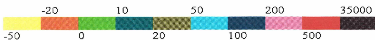
Map 13 :Difference of runoff between February 1978 and 1981 in WMO-region V
