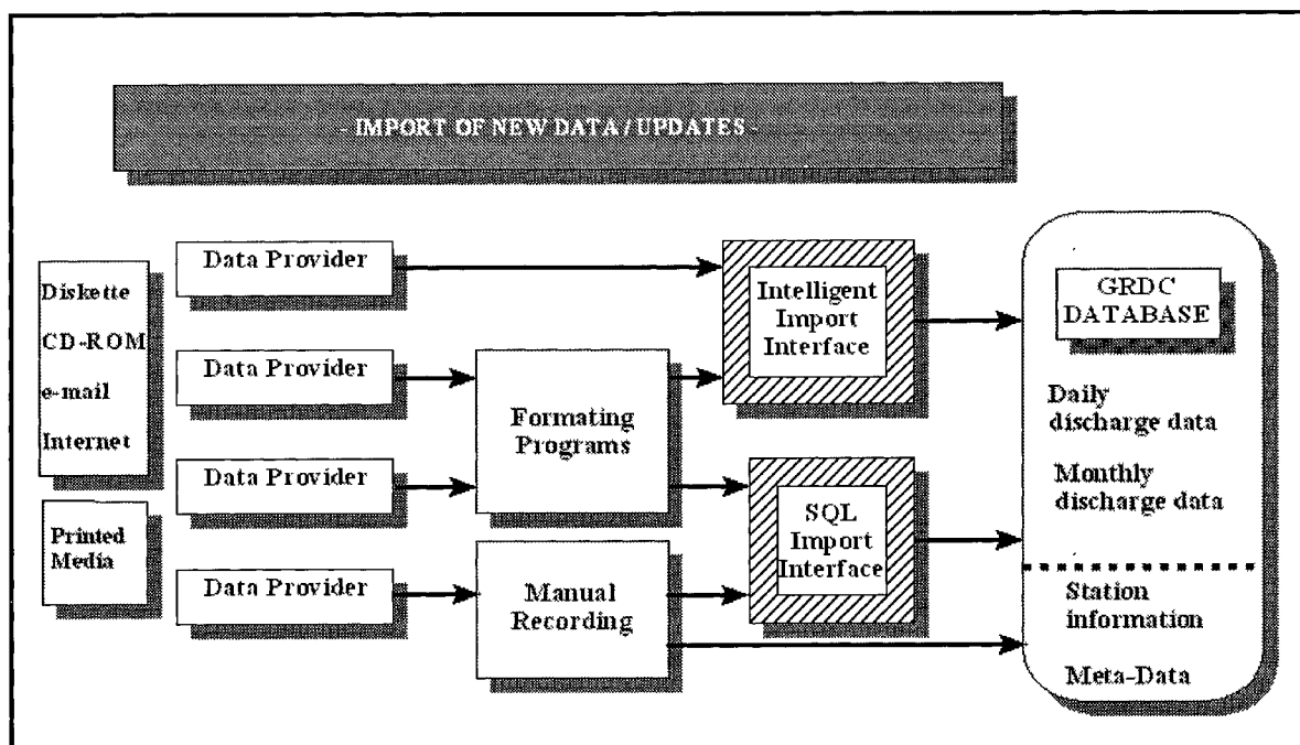
Figure 4: Dataflow Import
