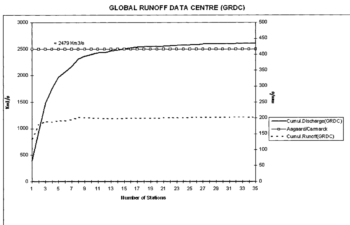
Fig. 1: Cumulated discharge and runoff of 35 stations from GRDC in comparison with volumesum of 9 stations from Aagaard and Carmack
