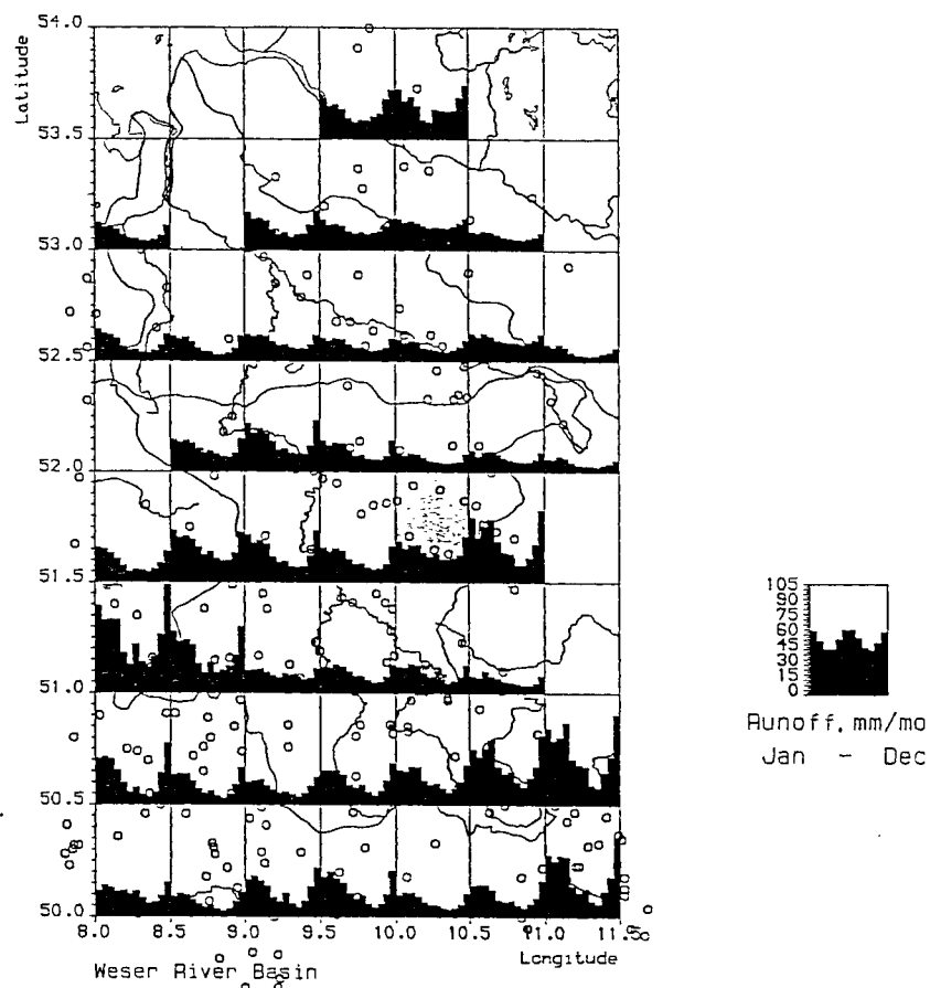
Fig. 1: Gridnet 0.5^\circ \times 0.5^\circ of the Weser Catchment, Germany, location of stream gauges, and histograms of mean monthly runoff within each grid cell, 1971 - 1980
