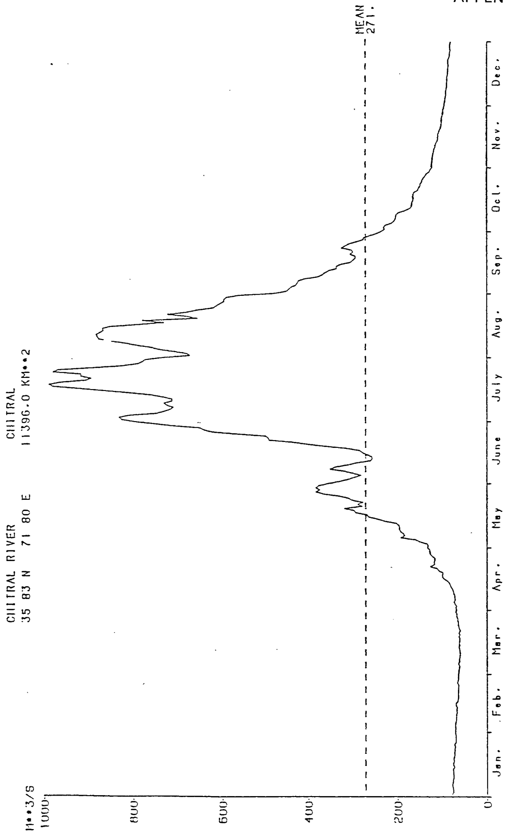
Figure 10: Mean Daily Discharge 1981
